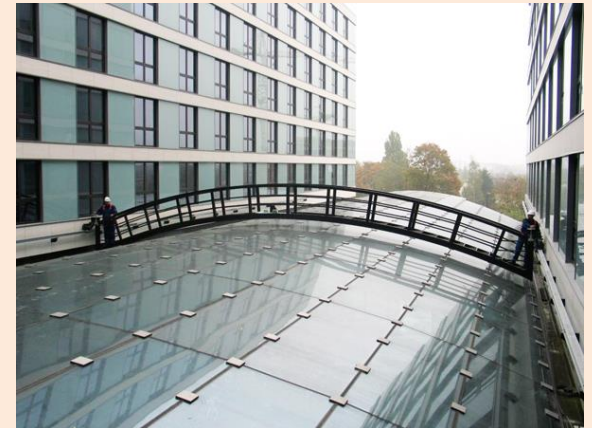
Gantry cradle for Danpalon roof maintenance
